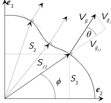
Fig. 1.7: Lamb mode slowness surface cut and group velocity at fixed frequency, \theta is the steering angle.
