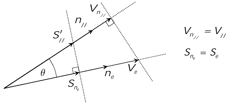
Figure 3.1 : Phase and energy slowness and velocity projection for non-dispersive plane waves. n_{//} is the phase direction, n_e is the energy direction.
