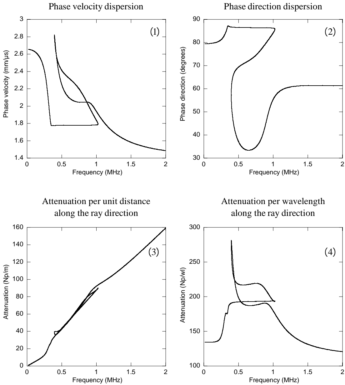
Figure 3.8: Frequency dispersion of the parameters of the S_0 mode, whose energy travels along the 50 degrees observation direction. The phase velocity dispersion is displayed in plot (1), the phase direction dependence on the frequency is displayed in (2), the attenuation per meter and per wavelength are respectively shown by plots (3) and (4).
