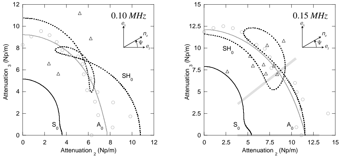
Figure 4.17: Experimental measurements and theoretical predictions of attenuation of fundamental guided modes. The horizontal axis is the direction of the fibres. Consistently with Figs.(4.14) and (4.15) the 0 and 40 degrees directions are shadowed.
