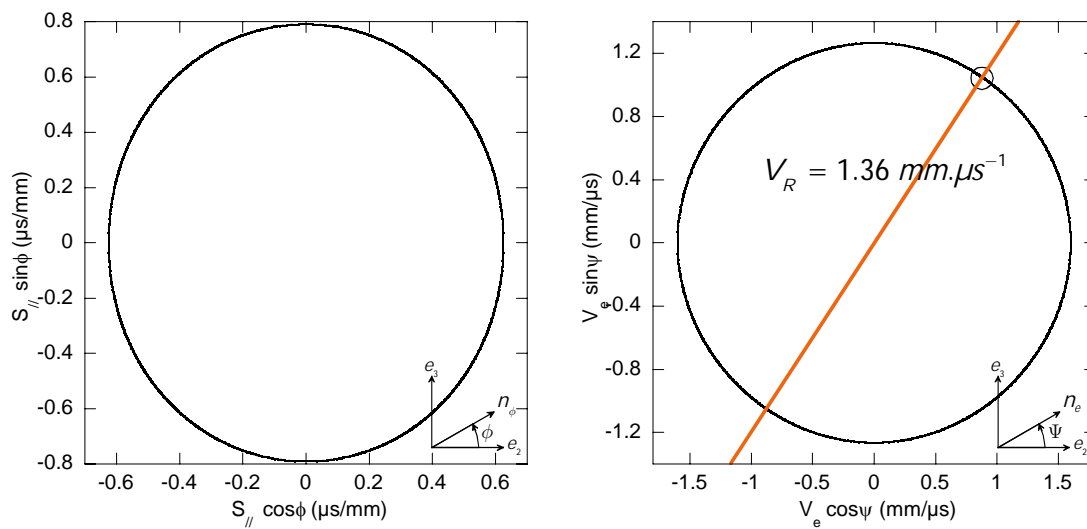
Figure 3.11: The Rayleigh slowness surface and wave surface in the carbon-epoxy material. At 50 degrees, direction indicated by the solid line, the energy velocity of the Rayleigh wave is 1.36 \text{ mm} \cdot \mu\text{s}^{-1} .
