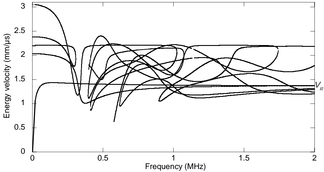
Figure 3.10: SH_0 , S_0 , A_0 , A_1 , S_1 and S_2 energy velocity versus frequency for the 50 degrees direction of observation, in the unidirectional carbon-epoxy plate.
