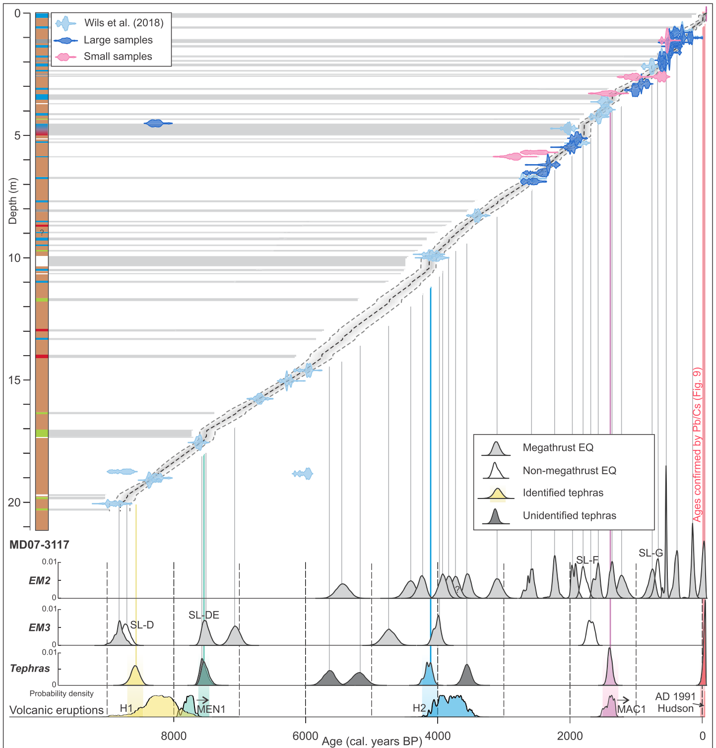
Figure 8. Radiocarbon-based age-depth model of MD07-3117 (95% confidence interval with mean age indicated by black dashed line) showing the age distributions for all tephras and seismo-turbidites identified in the core. Ages of large individual samples are indicated in shades of blue: those that were already measured by Wils et al. (2018) in light blue, new samples in dark blue. Small samples are indicated in pink. The most recent earthquake (EQ) and tephra ages are confirmed by short-lived radionuclide dating (see Figure 9). Age distributions of major Holocene eruptions (H1, MEN1, H2, MAC1, and the AD 1991 Hudson eruption) dated onshore are indicated on the lowermost age axis (Naranjo & Stern, 1998, 2004; Stern & Weller, 2012) and are correlated to their corresponding deposits in the core (verified by geochemical analysis in Wils et al., 2018, or this research) by color coding. Adapted from Wils et al. (2018).
