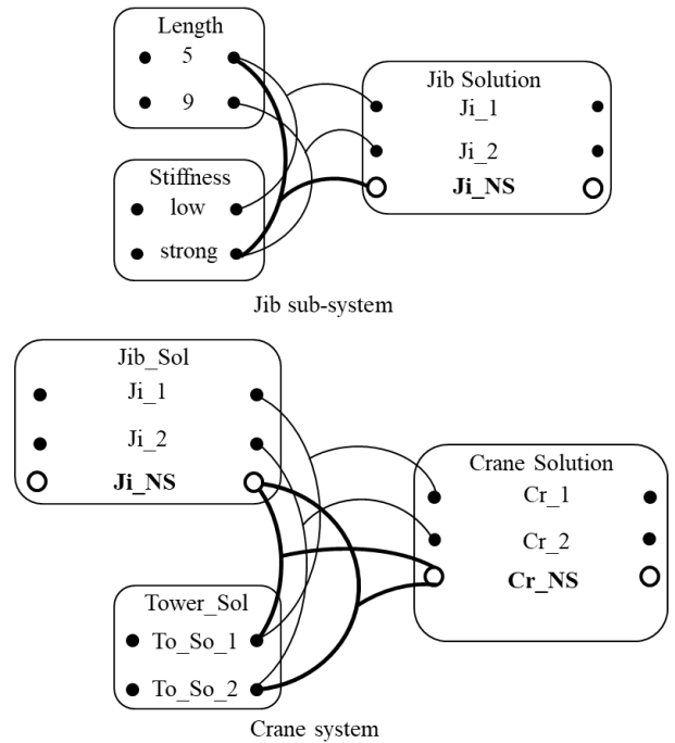
Figure 3: System configuration model in ETO situations
