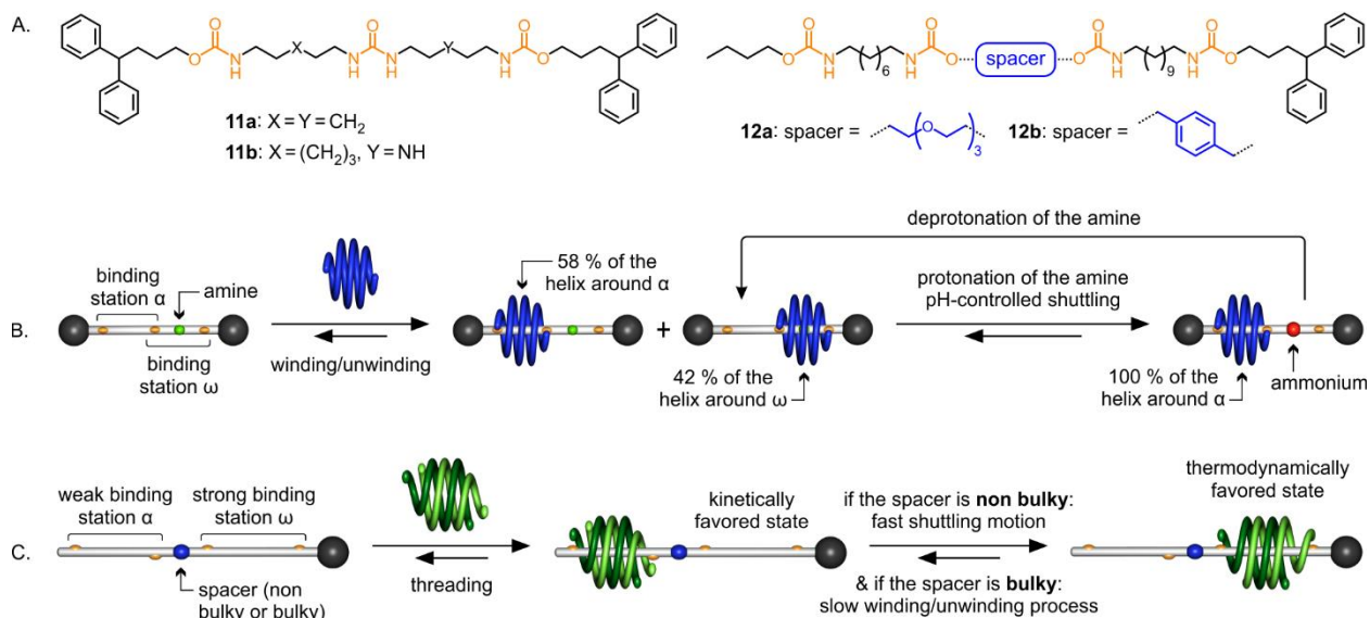
Figure 6. (A) Formulae of rods 11a-11b and 12a-12b . (B) Equilibria that govern the pH-controlled shuttling of single helix 2c (blue) along rod 11b . (C) Unidirectional fast shuttling (with a non-bulky spacer) or slow unwinding/rewinding (with a bulky spacer) of double helix (8c) 2 (green) from the \alpha -station to the \omega -station of rods such as 12a (tetraethylene glycol spacer) or 12b ( p -xylyl spacer).
