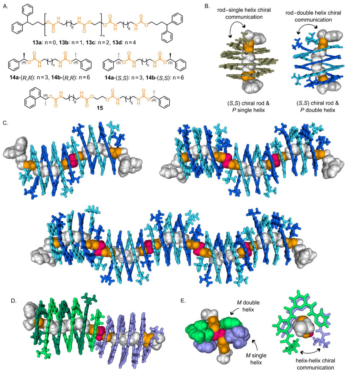
Figure 7. (A) Achiral rods 13a-13d and chiral rods 14a-14b and 15 . (B) Crystal structures of P - 2c \supset 14a-(S,S) (left) and P - (8b) 2 \supset 14b-(S,S) (right) showing rod-to-helix chirality induction. (C) Crystal structures of poly-foldaxanes (8b) 4 \supset 13b (top, left), (8b) 6 \supset 13c (top, right) and energy-minimized molecular model, using MMFFs, of the [11]foldaxane (8b) 10 \supset 13d (bottom). (D) Crystal structure of the homochiral [4]foldaxane M - (8c) 2 \cdot M - 2d \supset 15 with a zoomed view of the
