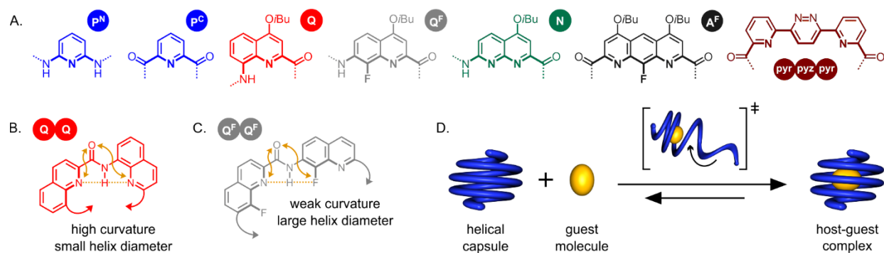
Figure 2. (A) Toolbox of heterocyclic amino acid, diacid or diamine aromatic building blocks of helical aromatic oligoamide foldamers, and their letter and color code. Folding principles of (B) Q 2 and (C) Q F 2 . Aryl-amide pseudo-conjugation, hydrogen bonds (dashed lines) and electrostatic repulsions (arrows) contribute to the stabilization of a preferred conformation at each aryl-amide bond, giving rise to a helix in sufficiently long sequences. Intramolecular aromatic stacking comes as an additional, solvent dependent, stabilizing force. (D) Encapsulation of a guest molecule (yellow sphere) in a molecular helical capsule (blue tube) possessing a reduced diameter at both ends, leading to a host-guest complex via a transient local unfolding of the helix.
