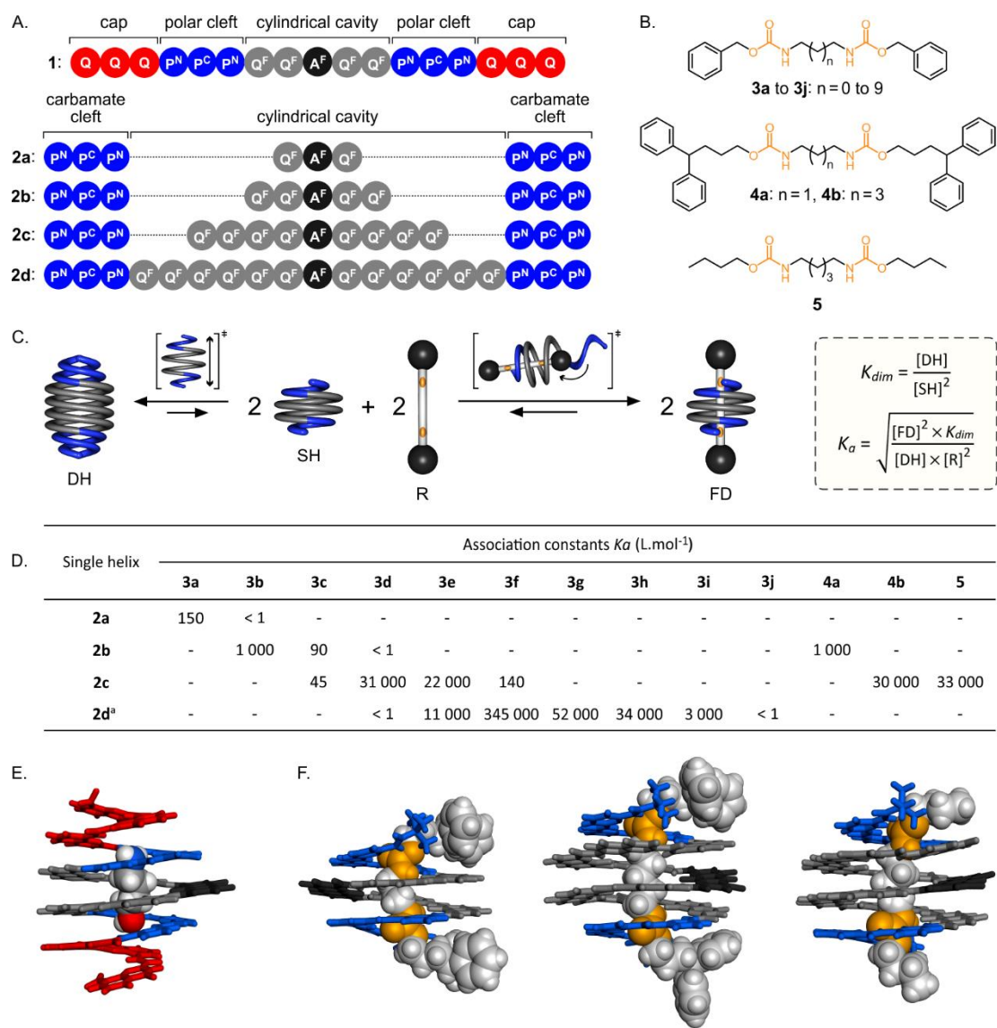
Figure 3. (A) Sequences 1 and 2a-2d. (B) Formulae of rod-like guests possessing two carbamate functional groups (orange) with bulky end groups (3a-3j, 4a-4b) or without (5). (C) Equilibria between a dumbbell-shaped rod (R), a single (SH) or double (DH) helical foldamer and a foldaxane (FD). (D) K_a values in CDCl 3 at 318 K of various foldaxanes and one pseudo-foldaxane, as determined by 1 H NMR spectroscopy. Crystal structures of complexes (E) 1 ⊃ 4-amino-1-butanol and (F) 2b ⊃ 4a, 2c ⊃ 4b and 2c ⊃ 5, from left to right. a For a homogeneous presentation, association constants ( K_a ) for 2d have been recalculated at equilibrium using the equation proposed in C.
