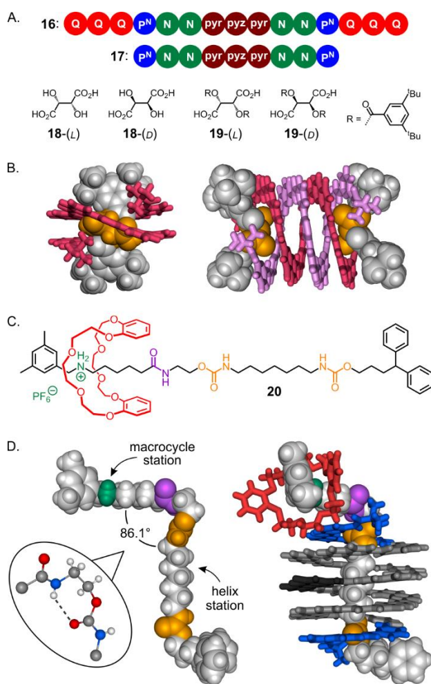
Figure 8. (A) Sequences of 16 and 17 and formulae of 18 and 19 . (B) Energy minimized molecular model, using MMFFs, of M - 17 ⊃ 19-(L) (left) and crystal structure of ( P - 17 ) 2 ⊃( 19-(L) ) 2 (right). Tartaric acid moieties and bulky end groups are represented in orange and grey, respectively. (C) Formula of [2]rotaxane 20 . (D) Crystal structure of the foldarotaxane 2d ⊃ 20 comprised of a DB24C8 macrocycle around an ammonium moiety and helix 2d wrapped around a dicarbamate
