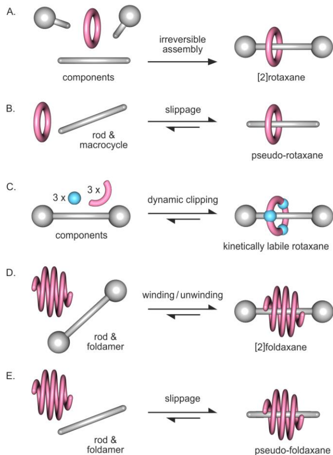
Figure 1. (A) Irreversible formation of a [2]rotaxane and (B-D) reversible formation of various types of architectures: pseudo-rotaxanes (B), kinetically labile rotaxanes (C), foldaxanes (D) and pseudo-foldaxanes (E).
