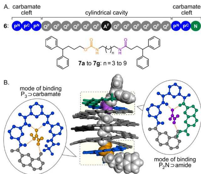
Figure 4. (A) Sequence of dissymmetrical helical foldamer 6 and formulae of dissymmetrical guests 7a-7g . (B) Crystal structure of 6 ⊃ 7c with zooms on the binding modes between either the P N P C P N cleft to the carbamate of the guest (left) or P N P C N to the amide (right).
