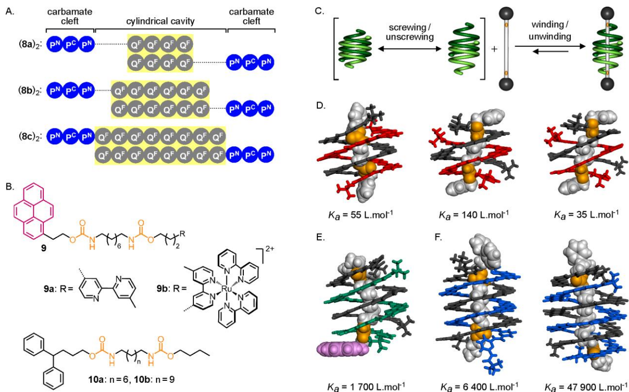
Figure 5. (A) Sequences of double-helical foldamers (8a)_2 - (8c)_2 . (B) Formulae of dicarbamate guests. Guest 9b is terminated by pyrene and Ru(bpy) 3 2+ chromophores (hexafluorophosphate counter anions are omitted for clarity). Guest 9a is its precursor. Guests 10a-10b possess only one bulky end group and thread themselves in double helix (8c)_2 . (C) Formation of a [3]foldaxane from a double helix (green) wrapped around anchor points (orange) of a dumbbell-shaped rod. Crystal structures and association constants in CDCl 3 of foldaxanes (D) (8a)_2 \supset 3b , (8a)_2 \supset 3d and (8a)_2 \supset 3e (left to right), (E) (8b)_2 \supset 9a and (F) (8c)_2 \supset 10a and (8c)_2 \supset 10b (left to right). Double helices (8a)_2 , (8b)_2 and (8c)_2 are shown in red/black, green/black and blue/black, respectively.
