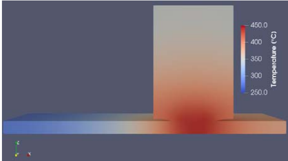
Fig. 6 Temperature distribution in the system, under 3000 rpm and 465 N (with ramp) during 500 s
