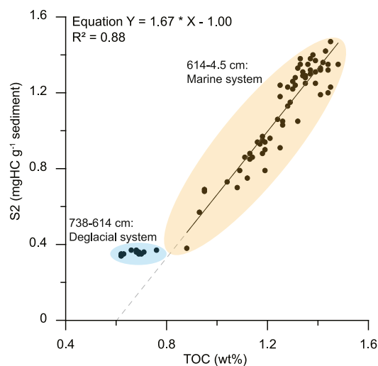
Fig. 6. The linear correlation between the S2 and TOC in the marine system shows that the regression line intercepts at 0.6 wt% TOC.
