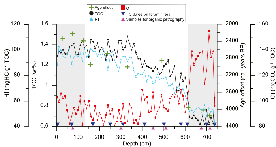
Fig. 3. Hydrogen Index (HI), TOC, age offset between bulk organic matter ^{14}\text{C} dates and the age model based on ^{14}\text{C} dates of mainly benthic foraminifera, intervals sampled for organic petrography and Oxygen Index (OI) plotted against core depth of the marine sediment core AMD14-204C. The grey and white boxes illustrate the three-part division of the record.
