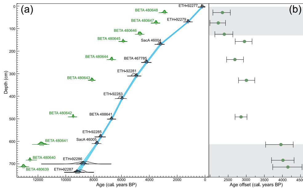
Fig. 2. (a) Age-depth model of the marine sediment core AMD14-204C, based on mainly mixed benthic foraminifera (grey age distributions; the light shaded area for each radiocarbon date illustrate the probability distribution before age modelling, while the darker grey areas represent the probability distribution after age modelling. The modelled age is shown in blue, with the envelope representing the modelled 1\sigma range) (Hansen et al., 2020). The bulk organic matter dates are plotted in green (Girardeau et al., 2020). (b) Age offsets between median calibrated bulk dates and the corresponding modelled age for each depth interval with 2\sigma uncertainties, calculated based on the 2\sigma age ranges derived from the age modelling. The grey and white boxes illustrate the three-part division of the record.
