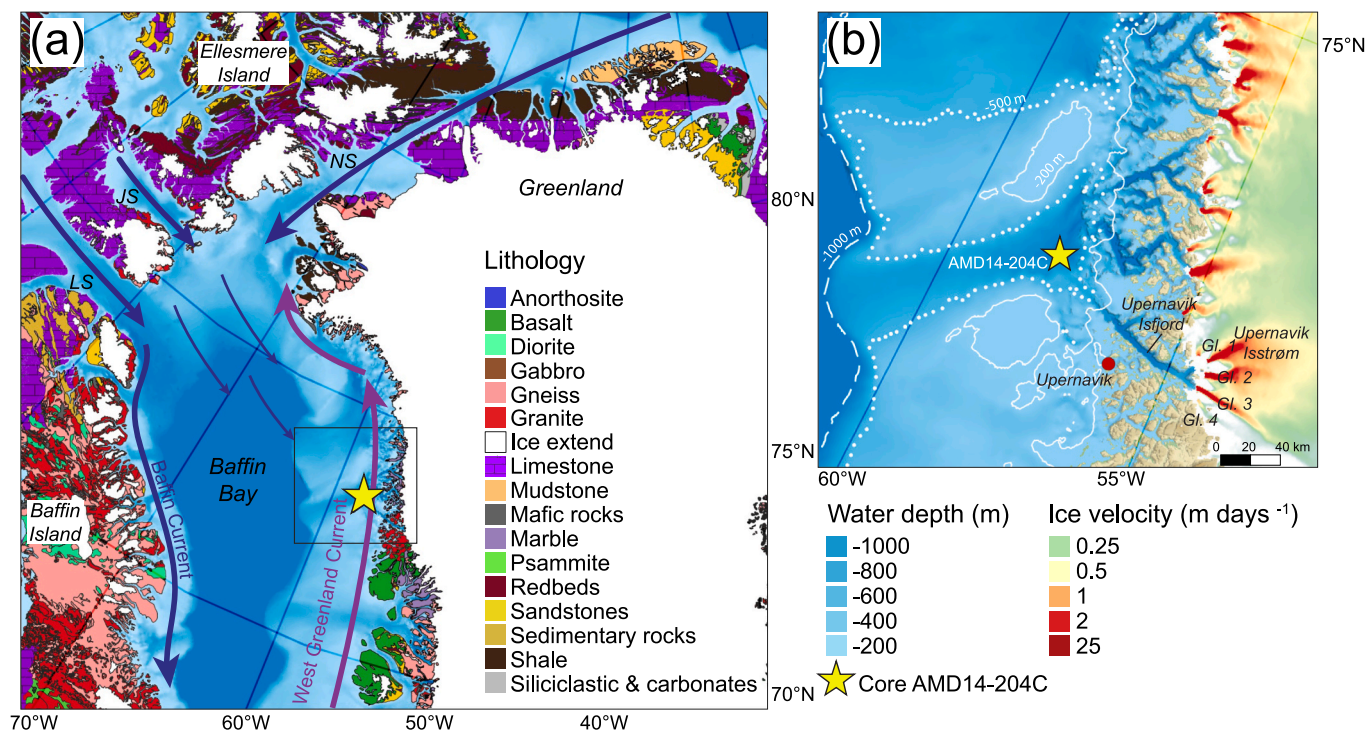
Fig. 1. (a): An overview of the geology of Baffin Island, Ellesmere Island and northwestern Greenland, modified after Harrison et al. (2011), together with modern ocean surface currents and study site. Purple and blue arrows indicate intermediate and cold water temperatures, respectively. LS = Lancaster Sound, JS = Jones Sound, NS = Nares Strait. (b) Zoom in on area defined by the black box in panel (a), showing the Upernavik Isfjord and Isstrøm, comprising four glaciers. Ice velocity data is derived from Sentinel-1 SAR data acquired from 2017 to 12-28 to 2018-02-28 (Nagler et al., 2015). Ocean bathymetry and bed topography data is derived from GEBCO and BedMachine v3 (Morlighem et al., 2017; Weatherall et al., 2015).
