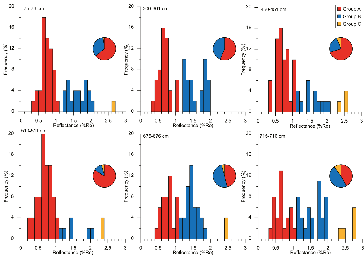
Fig. 5. The distributions and percentage frequencies of the counted organic vitrinites (groups A and B) and inertinites (group C) in the samples from various depths shown both as histograms and pie charts.
