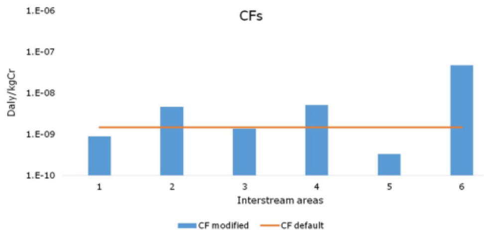
Fig. 8 The human health characterization factors - CF_{hum} (modified and default) of Cr in interfluve areas, soils [Daly/kgCr]. CF_{hum} default is the table value provided in the USEtox model. 1. Chulyum-Kiya, 2. Ob'-Chulyum-Kiya; 3. Chulyum-Ket'-Ulu-Yul; 4. Ob'-Chaya; 5. Ob'-Vasyugan-Chaya; 6. Chulyum-Ulu-Yul
