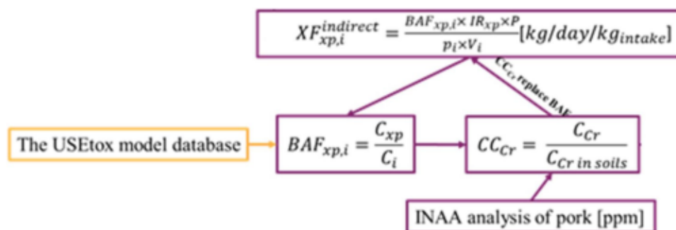
Fig. 1 The indirect exposure factor calculation (Fantke et al. 2017) and modification, (Belyanovskaya et al. 2019, 2020). XF_{indirect\ xp,i} , exposure factor; BAF_{xp,i} , bioaccumulation factor; IR , individual ingestion rate of a food substrate corresponding to exposure pathway xp ; P , population head count; p_i , bulk density of medium i [ kg/m^3 ], V_i , volume of medium i linked to the exposure pathway xp BAF_{xp,i} ,
