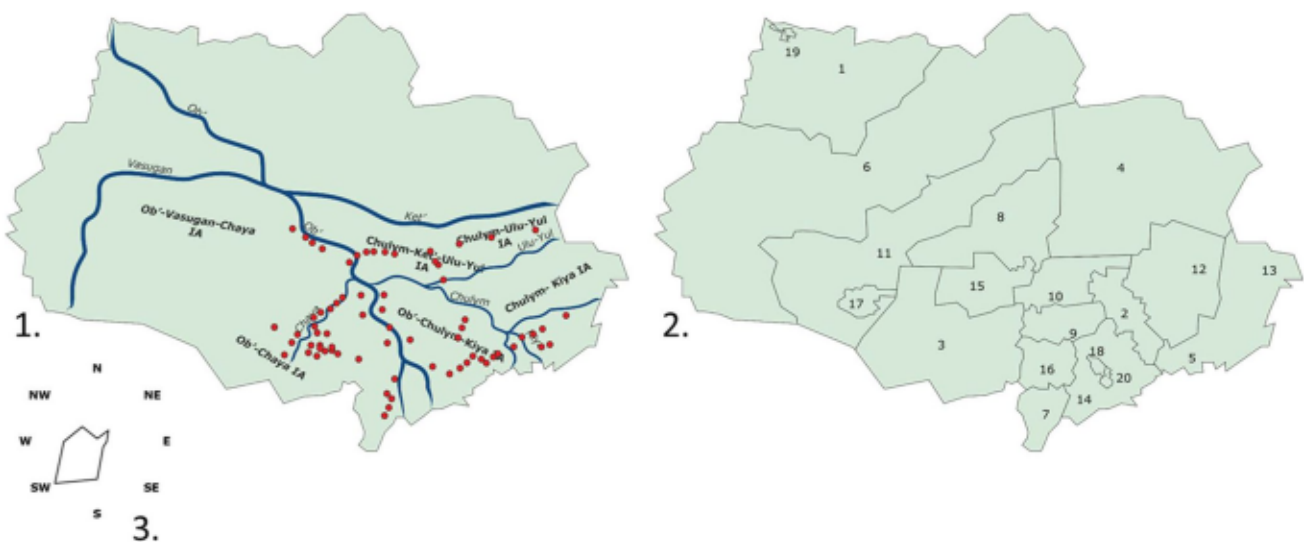
Fig. 2 The map of Tomsk oblast' with interfluvial areas (1), administrative map (2), and wind destination (3) ("Archive of weather in Tomsk," 2020) Note: Districts: 1. Aleksandrovskiy; 2. Asinovskiy; 3. Bakcharskiy; 4. Verkhneketskiy; 5. Zyryanskiy; 6. Kargasokskiy; 7. Kozhevnikovskiy; 8. Kolpashevskiy; 9. Krivosheinskiy; 10. Mol-
