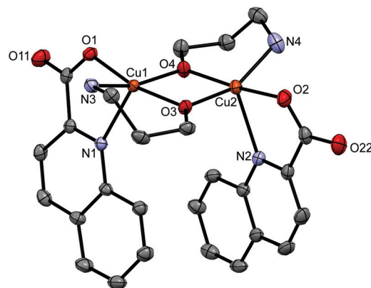
Fig. 4 ORTEP drawing of \text{syn}[\text{Cu}_2(\text{quin})_2(3\text{a}1\text{pO})_2] ( syn-11d ). Displacement ellipsoids are drawn at the 50% probability level. Hydrogen atoms are omitted for clarity.
