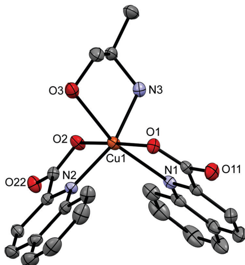
Fig. 2 ORTEP drawing of [\text{Cu}(\text{quin})_2(2\text{a}1\text{pOH})] ( 8b ). Displacement ellipsoids are drawn at the 50% probability level. Hydrogen atoms are omitted for clarity.
