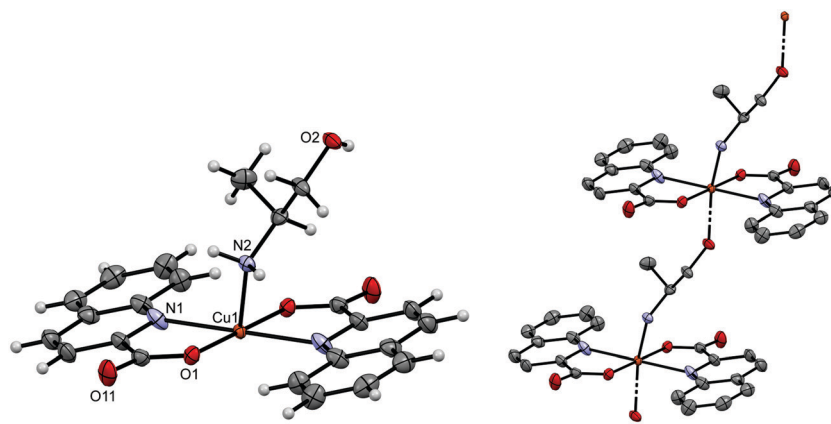
Fig. 3 ORTEP drawings of a repeating unit (left) and a short section of a chain (right) in [\text{Cu}(\text{quin})_2(2\text{a}1\text{pOH})]_n ( 8c ). The Cu(II) coordination sphere is completed by the O1, N1 and N2/O2 ( 1-x, 1-y, 1-z ) symmetry equivalents. Displacement ellipsoids are drawn at the 50% probability level. Hydrogen atoms are shown as spheres of arbitrary radii (left) or omitted for clarity (right).
