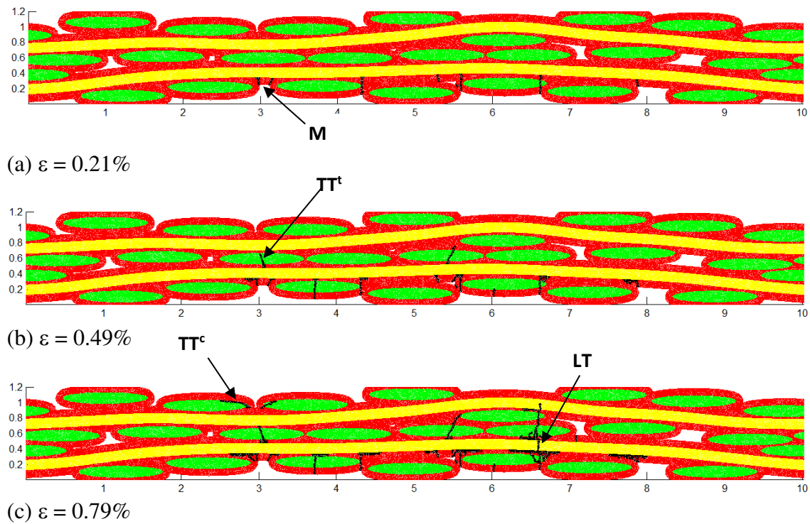
Fig. 8. The crack network resulting from the simulation of a bending test for three values of the relative deflection.
