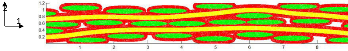
Fig. 4. Representation of the FE cell with a thickness t=1.2 mm and a length L=10 mm; the colors allow to identify each component including the matrix (red), the transverse (green) and the longitudinal (yellow) tows (For interpretation of the references to color in this figure legend, the reader is referred to the web version of this article). Direction 1 corresponds to the in plane warp direction and direction 2 is the thickness direction.
