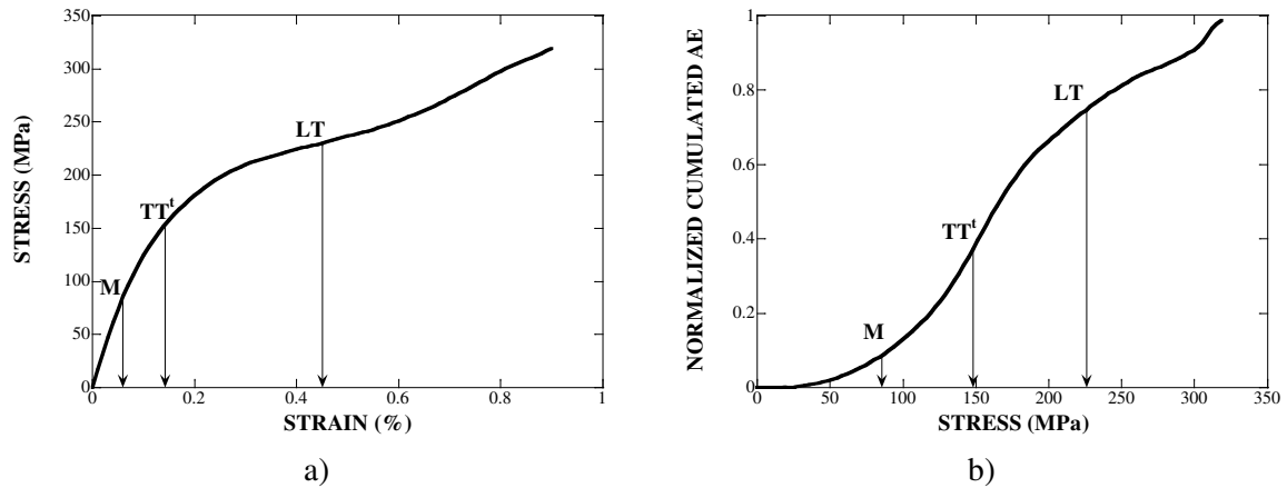
Fig. 3. Tensile testing of a SiC/SiC specimen: a) strain-stress response and b) cumulated AE (normalized by its maximum value) versus the applied stress. The onset (as revealed by in-situ observations) of the three main cracking mechanisms (matrix (M), transverse tows (TT t ), longitudinal tows (LT)) are indicated.
