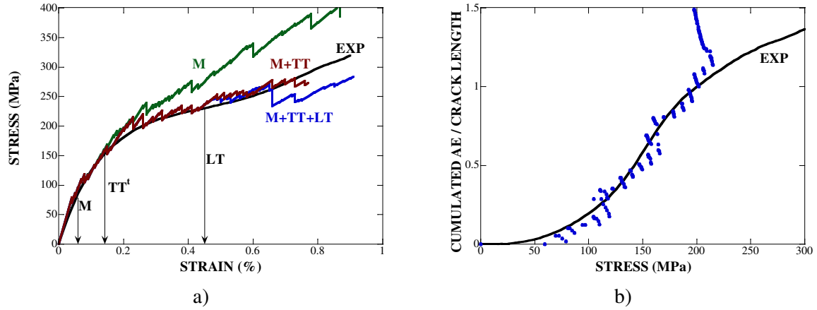
Fig. 7. Simulation of a tensile test and comparison with the experimental data: a) Strain stress response. The black curve is the experimental one and the colored ones are simulated responses (the green curve is obtained if only matrix cracking is considered), b) Cumulated acoustic emission (experimental) and cumulated crack length (simulated) versus the applied stress. The data are normalized by their maximum values reached for an applied stress of 200 MPa.
