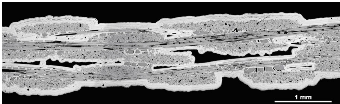
Fig. 1. Cross-sectional optical micrograph of a thin SiC/SiC composite elaborated by CVI [62]. White regions represent the SiC layers and the darker zones are SiC fiber bundles.
