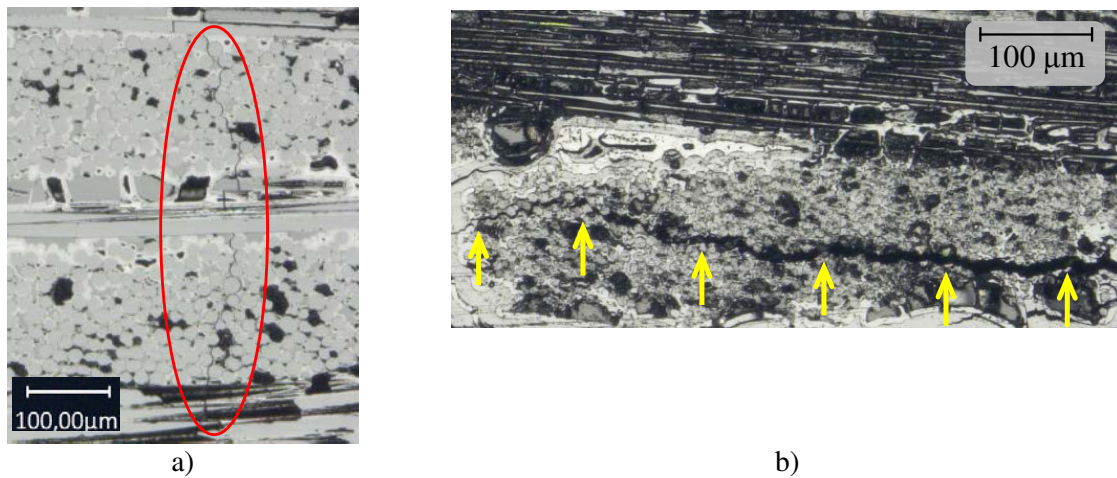
Fig. 2. Optical micrographs captured during mechanical testing of a thin SiC/SiC specimen [13] and revealing cracks in a) transverse tows under tensile test, b) a transverse tow under bending test (arrows indicate the crack generated by compressive failure). In each case, the direction of the applied load is horizontal.
