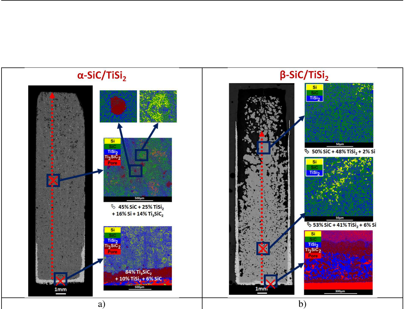
Figure 9. Optical and colored backscattered electrons images of the cross sections of the SiC compacts infiltrated by molten TiSi 2 at 1550°C for 1h: a) \alpha -SiC and \beta -SiC. The local surface fractions are given for whole image surface with an accuracy of \pm 5\% .
