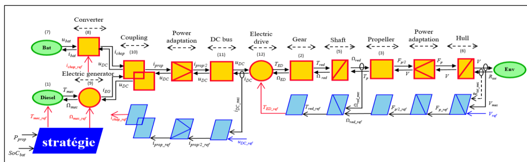
Figure 5: EMR of Hybrid Diesel - Battery Propulsion System
