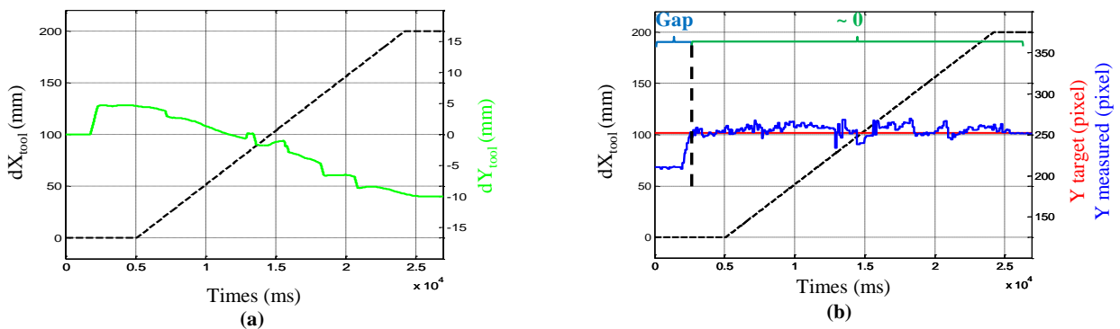
Figure 8. Visual control mode (a) Tool position along y-axis in millimeter (b) Tool position along y-axis in pixel on the image
