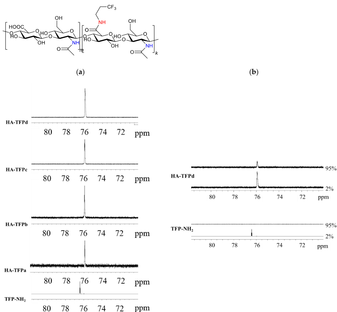
Figure 3. (a) 19 F NMR spectra of trifluoropropyl functionalized HA: HA-TFPa, HA-TFPb, HA-TFPc and HA-TFPd for initial molar ratios (NH 2 /COOH) = 10 (bottom), 20, 50, and 100 (top) %, respectively; TFP-NH 2 19 F spectrum is given as a reference (470.64 MHz, 318 K, DMSO- d 6 ). (b) One-dimensional (1D) diffusion-filtered 19 F NMR spectra of HA-TFPd and TFP-NH 2 with a gradient g of 2% and 95%.
