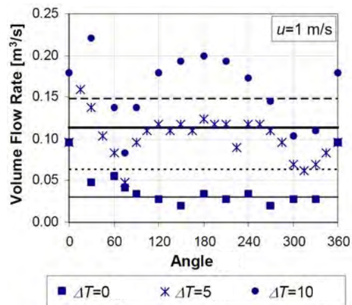
Figure 16 Measured and calculated volume flow rates: Warren & Parkins (black thin line), De Gids & Phaff (black dotted line, \Delta T = 0\text{ }^{\circ}\text{C} ), and De Gids & Phaff (black thick line, \Delta T = 5\text{ }^{\circ}\text{C} ) [54]
