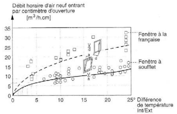
Figure 8 Variation of the airflow capacity of bottom and side hung windows as a function of the indoor-outdoor temperature [33]
