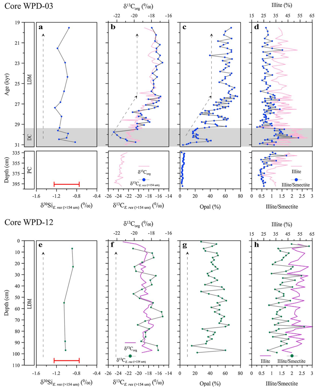
Figure 4. Age-depth profiles for \delta^{30}\text{Si}_{E, \text{rex}} , \delta^{13}\text{C}_{E, \text{rex}} , and \delta^{13}\text{C}_{\text{org}} ; opal content; and illite content and illite/smectite ratios in cores (a–d) WPD-03 and (e–h) WPD-12. The error bars in Figures 4a and 4e show the long-term external reproducibility ( \pm 0.25\text{‰} , 2\sigma_{\text{sd}} ) of the \delta^{30}\text{Si} measurements. The arrows in Figures 4a–4c and 4e–4g show general stratigraphic trends. Data in Figures 4a, 4e, 4f, and 4h are original to this study; data in Figures 4b–4d and 4g are from Xiong et al. [2012a, 2012b, 2013a]. LDM: laminated E. rex diatom mats, DC: diatomaceous clay, and PC: pelagic clay.
