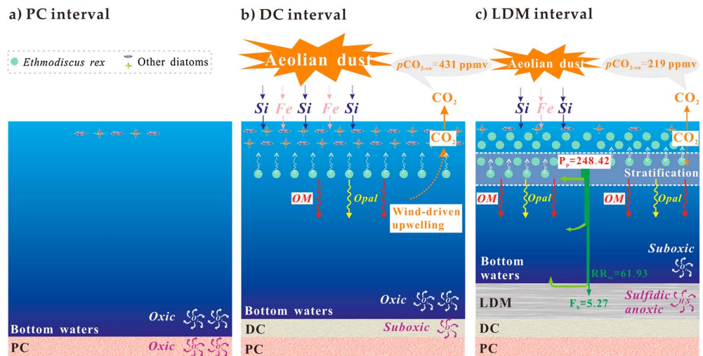
Figure 8. Schematic model of relationship of laminated E. rex diatom mat formation to paleoceanographic conditions in the EPS during the LGM: (a) PC interval, (b) DC interval, and (c) LDM interval. Inferred benthic redox conditions are from Xiong et al. [2012b]; patterns of dust input, wind-driven upwelling, and thermohaline stratification are from Xiong et al. [2010, 2013a]; p\text{CO}_{2\text{-sw}} estimates are from Xiong et al. [2013a]; and productivity estimates are from Xiong et al. [2013b]. In Figures 8a–8c, the number of E. rex and other diatoms shown is proportional to their inferred productivity; the number of blue and pink arrows shown is proportional to the magnitudes of the Asian eolian silicon and iron fluxes, respectively; and the number of red and yellow arrows shown is proportional to the magnitudes of organic matter and opal sinking fluxes, respectively. Abbreviations: OM, organic matter; p\text{CO}_{2\text{-sw}} , \text{CO}_2 partial pressure of the study area surface waters; P_p , primary productivity; \text{RR}_{\text{oc}} , rain rate of organic carbon; F_b , burial flux of organic carbon; LDM, laminated E. rex diatom mats; DC, diatomaceous clay; and PC, pelagic clay. See section 4.4.3 for further explanation.
