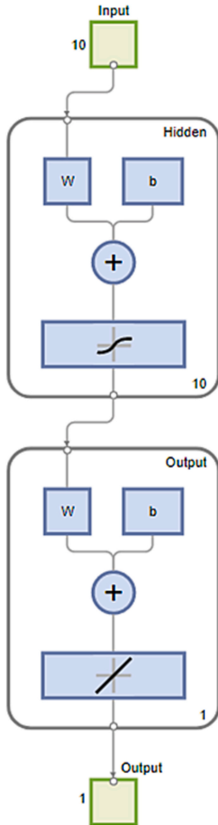
Fig. 5. Architecture of the FFN with 10 input variables and 10 nodes.
