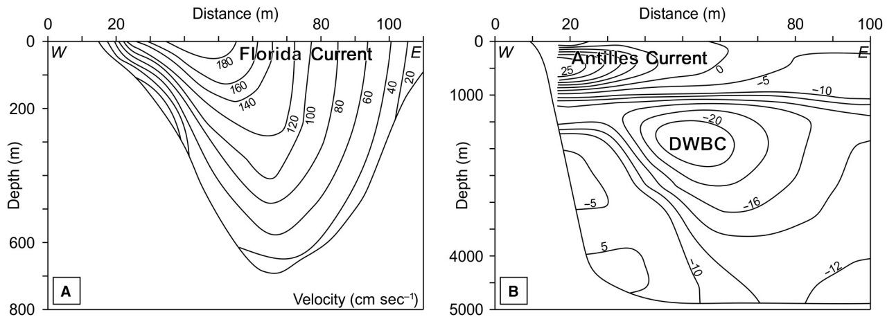
Fig. 3. Transects showing the superposed water masses (see Fig. 1 for location). (A) Florida Current (Johns et al. , 1995). (B) Deep Western Boundary Current (DWBC; Lee et al. , 1990).
