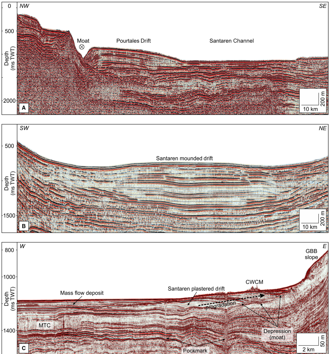
Fig. 4. (A) High-resolution seismic line through the Straits of Florida showing the geometry of the Pourtales Drift (see Fig. 1 for location; modified from Bergman, 2005). (B) High-resolution seismic line through the Santaren Channel showing the symmetrical mounded accumulation interpreted as the mounded or confined Santaren Drift (Lüdmann et al. , 2013; Fig. 1 for location; modified from Bergman, 2005). (C) High-resolution seismic line (Carambar cruise) along the toe of Great Bahama Bank slope showing the geometry of the Santaren Drift (from Principaud et al. , 2018; Fig. 1 for location). CWCM, cold water carbonate mounds; GBB, Great Bahama Bank; MTC, mass transport complex.
