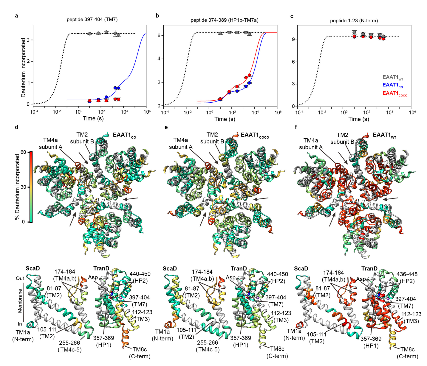
Figure 2. | Deuterium exchange at 20°C. (a-c) Deuterium uptake kinetics at 20°C of examples peptides from EAAT1 WT (grey), EAAT1 CO (blue), and EAAT1 COCCO (red), respectively, covering both helical and unstructured regions of the transporters. Solid lines represent double-exponential fits to the data, and dotted lines the expected deuterium kinetics of unfolded and solvent exposed peptides (see ‘HDX kinetic analysis’ in Methods). Plots in (a-c) depict an average of three independent experiments, and error bars represent s.e.m. (d-f) Deuterium incorporation after 1 hr at 20°C in EAAT1 CO (d), EAAT1 COCCO (e), and EAAT1 WT (f) mapped into the structure of the EAAT1 CRYTS (PDB 5LLM) trimer viewed from the extracellular medium (upper panel), as well as the scaffold (ScaD) and the transport (TranD) domains viewed from the membrane (lower panel), respectively. These domains are depicted separately for clarity of display, and black lines indicate the approximate position of some peptides in the structure, and the substrate (Asp). In the trimeric depiction, arrows point to the interface between protomers. Deuterium incorporation was calculated as an average of three independent experiments, and normalized to the maximal theoretical incorporation based on the number of backbone amide available for exchange in each peptide. The color code representing deuterium incorporation is depicted in a scale bar (d).
