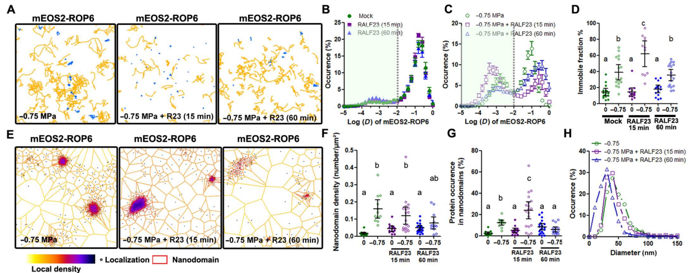
Fig. 5. RALF23/FER acts both on ROP6 diffusion and clustering. (A) Image reconstruction of several tens of single mEOS2-ROP6 molecule trajectories after RALF23 pretreatment of 15 or 60 min and followed by osmotic stimulation. Trajectories with low or high instantaneous diffusion coefficient in blue and yellow, respectively. Bimodal distribution of molecule instantaneous diffusion coefficient in control (B) or after osmotic stimulation (C) for plants expressing mEOS2-ROP6 in the absence (green circle), 15-min (purple squared), or 60-min RALF23 pretreatment (blue triangle). (D) Histogram represents the percentage of molecules with an instantaneous diffusion coefficient below 0.01 \mu\text{m}^2 \text{s}^{-1} . (E) Voronoi tessellation of mEOS2-ROP6 molecule localization map after RALF23 pretreatment of 15 or 60 min and followed by osmotic stimulation. Color code represents the local density of each molecule (labeled as a black circle). Nanodomains are highlighted by a red circle. (F) Nanodomain density and (G) relative occurrence of mEOS2-ROP6 in nanodomains after RALF23 pretreatment of 15 or 60 min followed by osmotic stimulation. (H) Distribution of nanodomain diameters. Error bars correspond to the 95% confidence interval. ANOVA followed by Tukey test, letters indicate significant differences among means ( P < 0.01 ). n > 12 from at least two independent biological replica.
