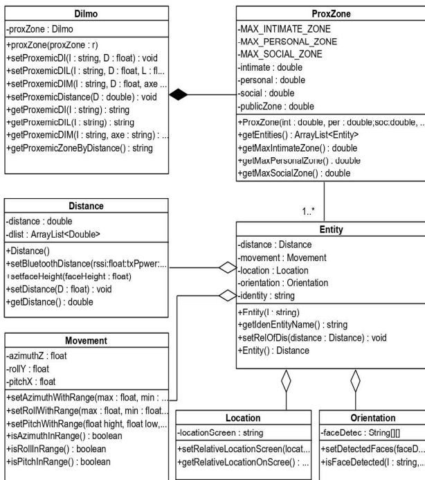
Figure 3. UML Class Diagram of the API.
