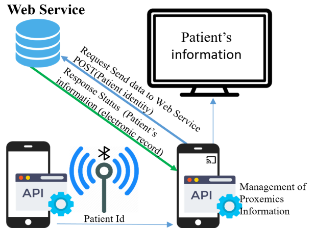
Fig. 1. Architecture to support development DILMO Mobile applications
