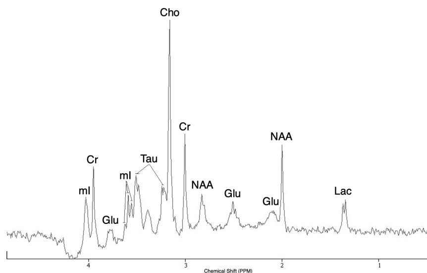
Figure 1. In vitro ^1\text{H} spectrum of the solution of 7 brain metabolites with a concentration fixed at 25 mM acquired with the microcoil (detection volume: 0.450\ \mu\text{L} ) at 7 T using the PRESS sequence (TR/TE = 2000/15 ms, Nacc = 256, Tacq = 8 min 32 s).
