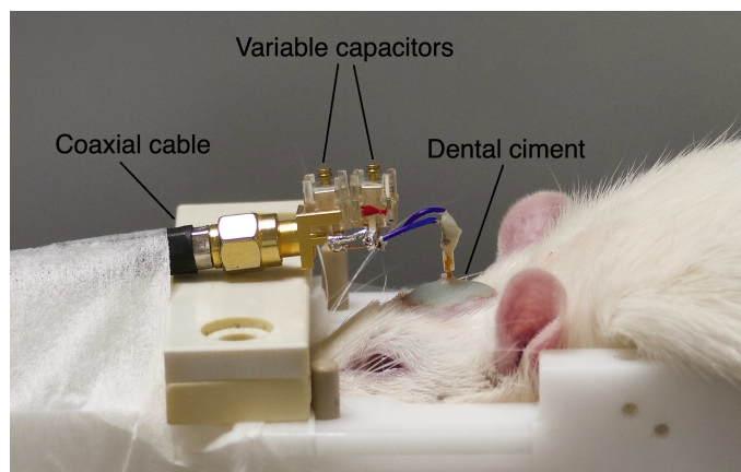
Figure 5. Illustration of the experimental set-up.
