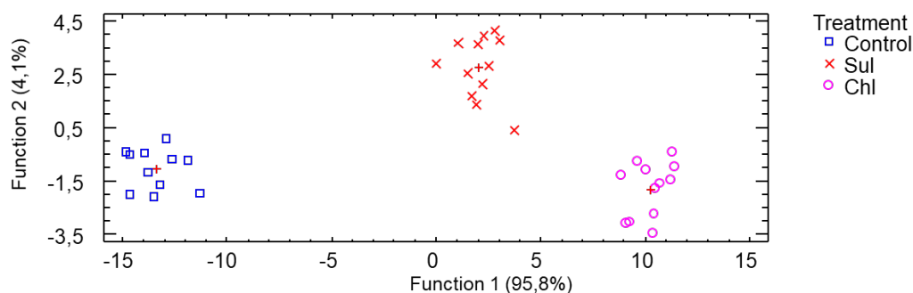
FIGURE 2. Distribution of grape samples in the two dimensional coordinated system by two first discriminant functions.
