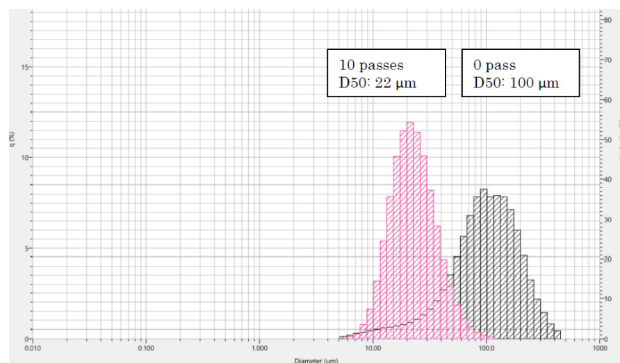
Figure 3. Particle size distribution of the fungal chitosan after 0 and 10 passes of treatment with high-pressure water jet system.
