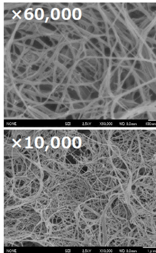
Figure 2. FE-SEM analysis of the fungal chitosan nanofibers (10 passes of treatment) obtained from the high-pressure water jet system (Star Burst Mini).
