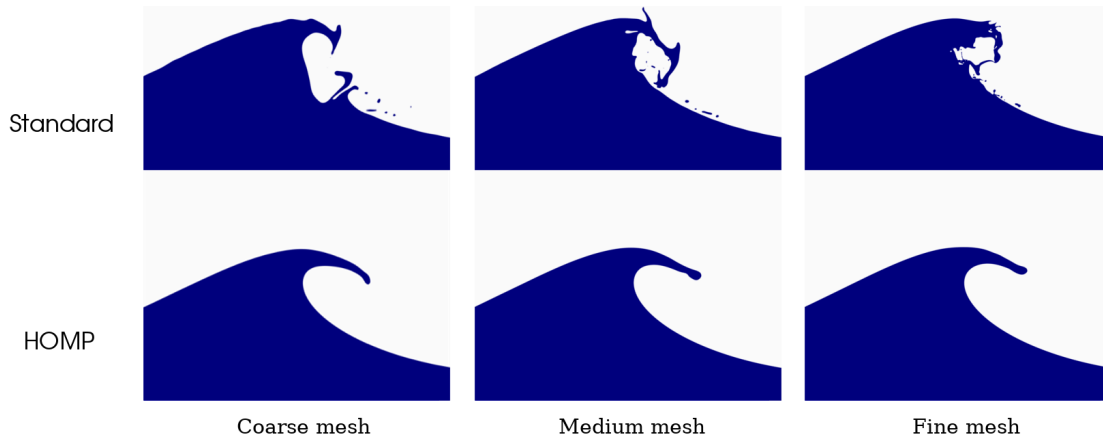
Figure 13: Plunging breaking wave: comparison of the breaking dynamics with the standard and proposed HOMP method using VOF-PLIC interface representation for every meshes (coarse, medium and fine). The interface thickness is reduced linearly with the spatial step.
