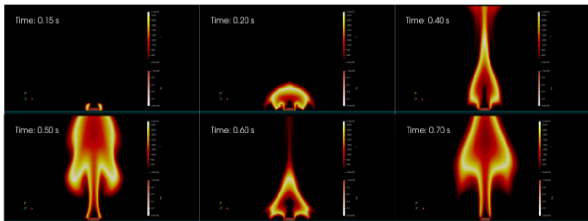
Figure 7. Starting of the fire. Six different snapshots to represent the initial evolution of the fire. At time t = 0.15 s two sparks are generated on the side of the wood log to trigger the combustion. A fire is generated and start propagating in the domain. By comparing the time t = 0.50 s with the time t = 0.70 s it is possible to observe the periodic behavior of the flame, the puffing effect.
