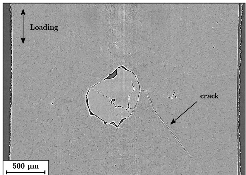
FIGURE 9 Tomographic slice (corresponding to the black line in Figure 6B) of the internal crack at the end of the initiation stage N = 1.84 \times 10^7 cycles (scan 1) on specimen S56 tested at PISCHE beamline of synchrotron SOLEIL
