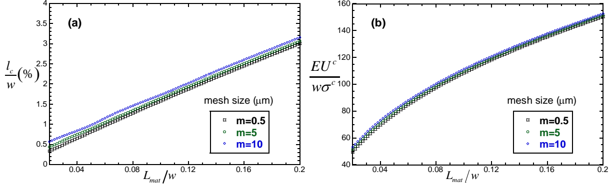
Figure 7: a) Initiation length and b) Applied displacement determined with the FFE approach versus the characteristic length for different values of the minimum mesh size m_{\text{FFE}} at the notch tip with M_{\text{FFE}} = 200\mu\text{m} . The three-point bending geometry with a sharp V-notch is considered with 2L = 40\text{mm} , w = 2\text{mm} , h = 0.3\text{mm} , \beta = 40\text{deg} . and E=400\text{ GPa} , \nu = 0.2 .
