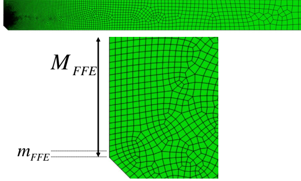
Figure 4: Refined mesh at the V-notch tip (FFE approach): the minimum mesh size and the length of the refined zone are respectively denoted m_{FFE} and M_{FFE} .
