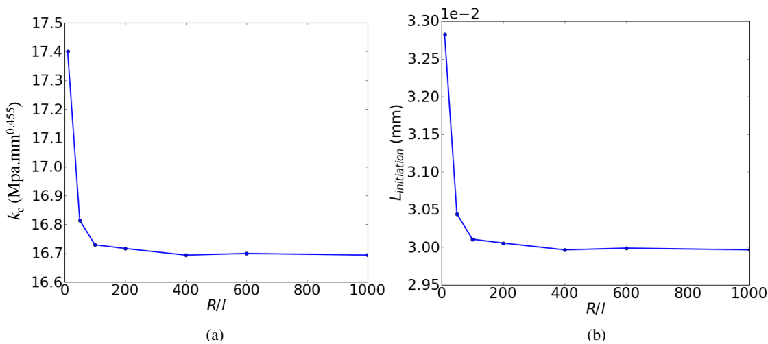
Figure 6: Initiation (a) critical stress intensity factor and (b) crack length determined with the MA approach as a function of the inner domain radius to crack length ratio for a sharp V-Notch with \beta = 90\text{deg.} , E = 3300\text{MPa} , \nu = 0.36 , \sigma_c = 72\text{MPa} and G_c = 0.250\text{MPa}\cdot\text{mm} . The minimum mesh size to crack length ratio is \frac{m_{MA}}{l} = 0.01 .
