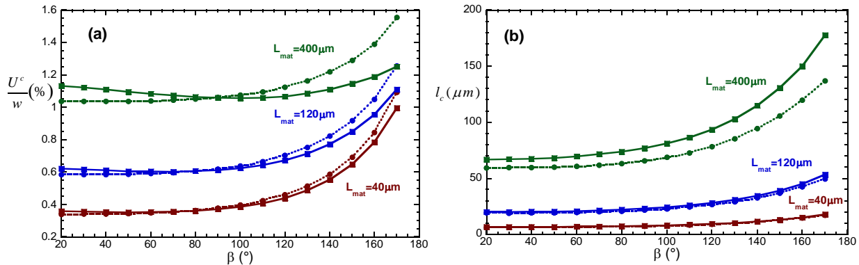
Figure 9: Comparison between MA (square symbols and full lines) and FFE (disk symbols and dotted lines) approaches: a) Applied displacement and b) Initiation length at crack onset versus the notch angle for various values of the characteristic length L_{\text{mat}} . A three-point bending specimen with a sharp V-notch is considered with 2L = 40 \text{ mm} , w = 2 \text{ mm} , h = 0.3 \text{ mm} and E=400 \text{ GPa} , \nu = 0.2 , \sigma^c = 100 \text{ MPa} and Gc=1, 3 \text{ or } 10 \text{ J/m}^2 corresponding to L_{\text{mat}}=40, 120, \text{ or } 400 \mu\text{m} .
