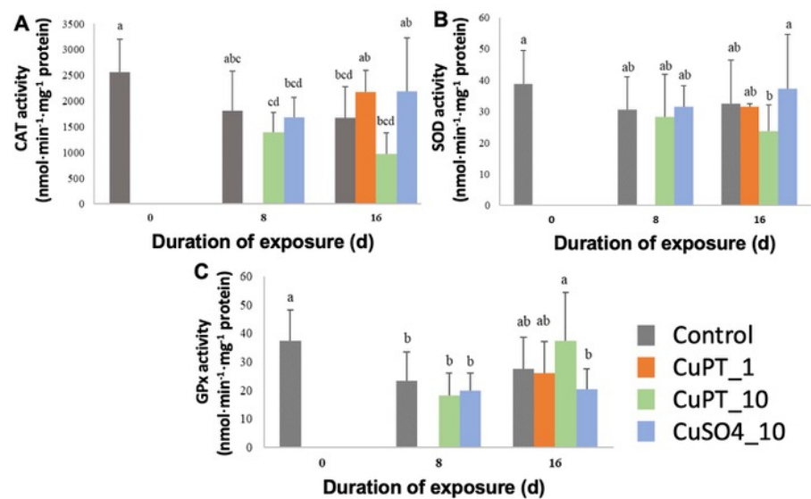
Figure 4 - Enzyme activities in liver of rainbow trout in nmol·min -1 ·mg -1 proteins for CAT (A), SOD (B), and GPx (C) depending on the duration of exposure to CuPT or CuSO 4 (n = 15, mean + SE). Different letters indicate a significant difference among conditions (Kruskal-Wallis followed by Mann-Whitney U test with Bonferroni correction, p <0.05), no data for CuPT_1 at Day 8.
