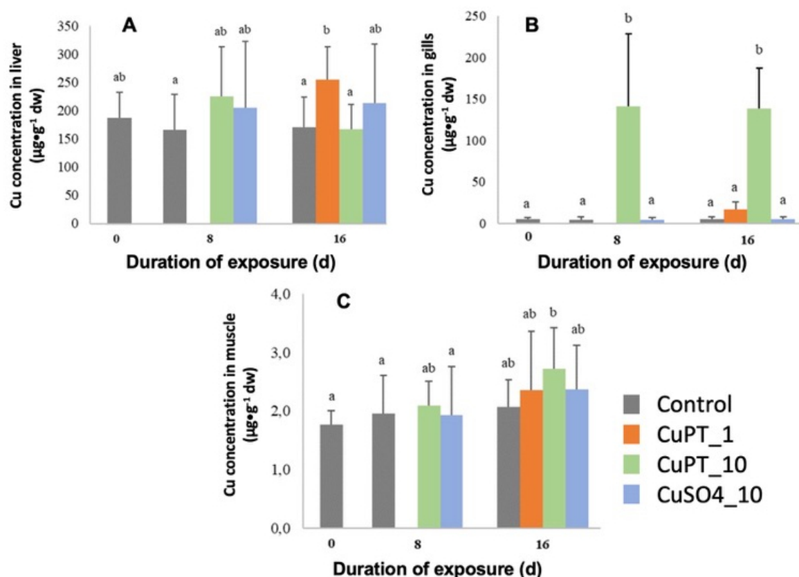
Figure 2 - Cu concentrations in liver (A), gills (B) and muscle (C) according to the duration of the exposure to CuPT or CuSO 4 ( \mu\text{g}\cdot\text{g}^{-1} dw) ( n = 15 , mean + SE). Different letters indicate a significant difference among conditions (Kruskal-Wallis test followed by Dunn's test; p < 0.05 ).
