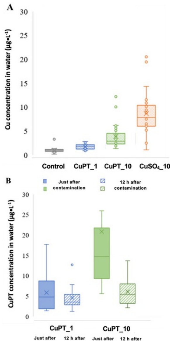
Figure 1 - Boxplot of the gross values of Cu (A, n=15 ) and CuPT (B, n=10 ) concentration in water ( \mu\text{g}\cdot\text{L}^{-1} ) on the sampling days for the different conditions of exposure to CuPT and CuSO 4 . For Cu analyses: boxplot of all the values (just after contamination and 12 h after contamination, combined) for control (grey, n=24 ), CuPT_1 (blue, n=30 ), CuPT_10 (green, n=26 ) and CuSO 4 (orange, n=26 ). For CuPT analyses: boxplot of the values just after contamination ( n=13 ) and 12h after contamination ( n=13 ), same colours for CuPT_1 ( n=14 ) and CuPT_10 ( n=14 ).
