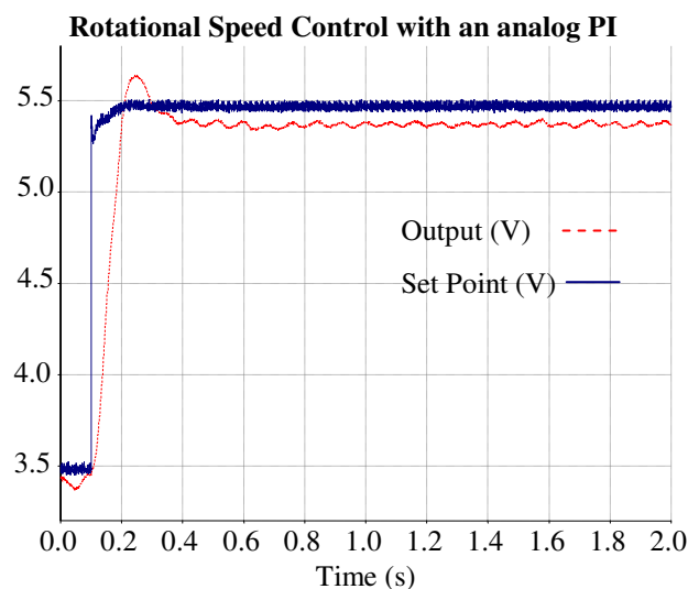
Fig. 8. Step response of the mechatronic process obtained with an analog PI controller
