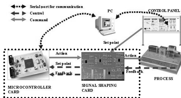
Fig. 5. Physical parts of the complete system
