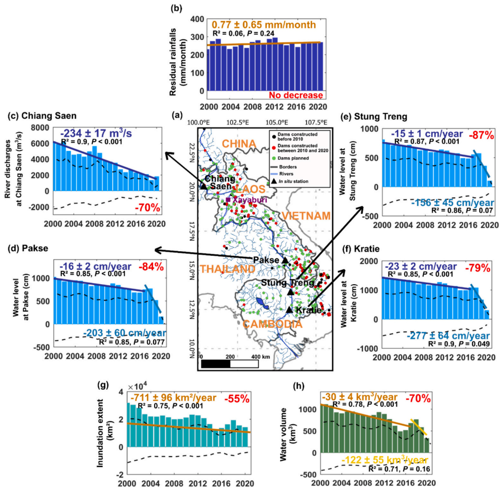
Fig. 7. Amplitude variations of the annual cycle (obtained by Census-X11 method) for surface water extent and volume, residual rainfall and comparison with in situ data. a) Map of the Mekong Basin showing dams locations. Barplot of the amplitude of the annual cycle using the Census-X11 decomposition for b) residual rainfall calculated using the difference between rainfall and evapotranspiration, c) river discharges ( \text{m}^3/\text{s} ) at Chiang Saen, water level (m) at d) Pakse, e) Stung Treng and f) Kratie, respectively, and for g) inundation extent ( \text{km}^2 ) and h) water volume ( \text{km}^3 ). For each barplot, dotted black points show minimum and maximum values of the cycle, blue (dark and light), orange and yellow straights are trends of the amplitude variations. Dams information came from https://monitor.mekongwater.org .
