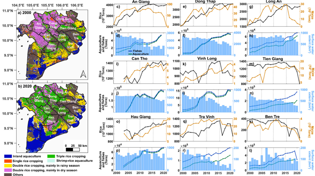
Fig. 9. Land use changes in the Vietnamese Mekong delta and time series of rice and maize production, aquaculture, fisheries and amplitude of surface water extent in nine provinces (An Giang, Dong Thap, Long An, Can Tho, Vinh Long, Tien Giang, Hau Giang, Tra Vinh and Ben Tre) over 2000–2020. a) land use map in 2000 with seven classes (inland aquaculture, single rice cropping, double rice cropping in rainy and dry seasons, triple rice cropping, shrimp-rice cropping, others (from Vu et al., 2022a), b) land use map in 2020 (from Vu et al., 2022b). Rice, maize, aquaculture, fisheries and amplitude of surface water extent are displayed for each province: c), d) for An Giang, e), f) for Dong Thap, g), h) for Long An, i), j) for Can Tho, k), l) for Vinh Long, m), n) for Tien Giang, o), p) for Hau Giang, q), r) for Tra Vinh, s), t) for Ben Tre.
