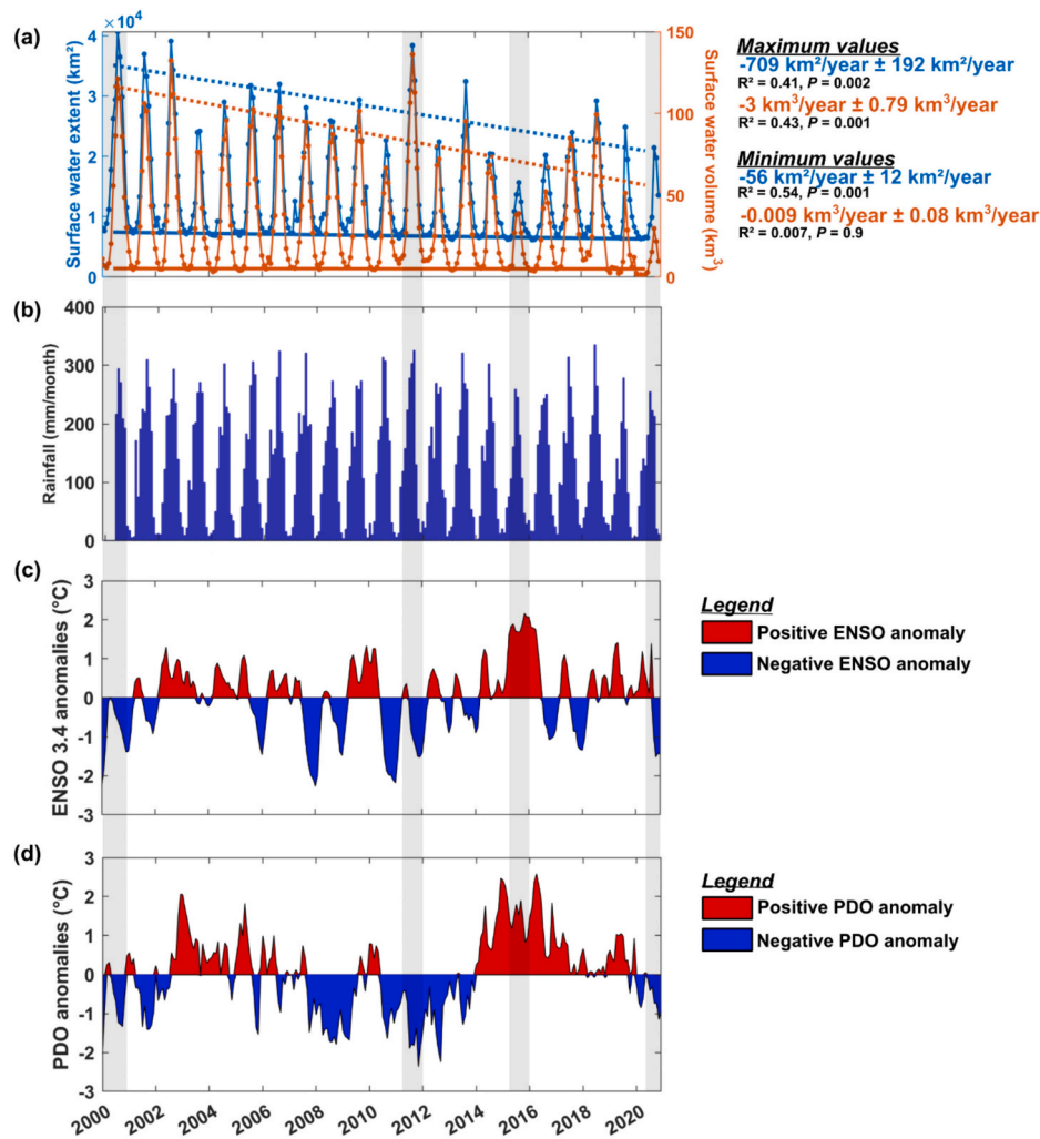
Fig. 3. Time series of the extent ( \text{km}^2 ) and volumes ( \text{km}^3 ) of surface water, rainfall (mm/month), and climatic indices ENSO and PDO anomalies ( ^{\circ}\text{C} ) over 2000–2020. a) Time series of surface water extent from multispectral imagery ( \text{km}^2 - blue) and surface water volumes ( \text{km}^3 - orange) over 2000–2020. For each time series, trend slopes of maximum values (dotted line) and minimum values (solid line) are displayed, -709 \pm 192 \text{ km}^2/\text{year} corresponds to a slope of -709 \text{ km}^2/\text{year} and a standard error of 192 \text{ km}^2/\text{year} with statistics ( R^2 is the coefficient of determination and P is the p -value), b) time series of rainfall data from GPM over 2000–2020, c) time series of anomalies of ENSO 3.4 and d) time series of PDO (Pacific Decadal Oscillation) indices anomalies over 2000–2020. Grey rectangles represent minimum and maximum values of inundation extent and surface water volumes, with rainfall, ENSO and PDO associated.
