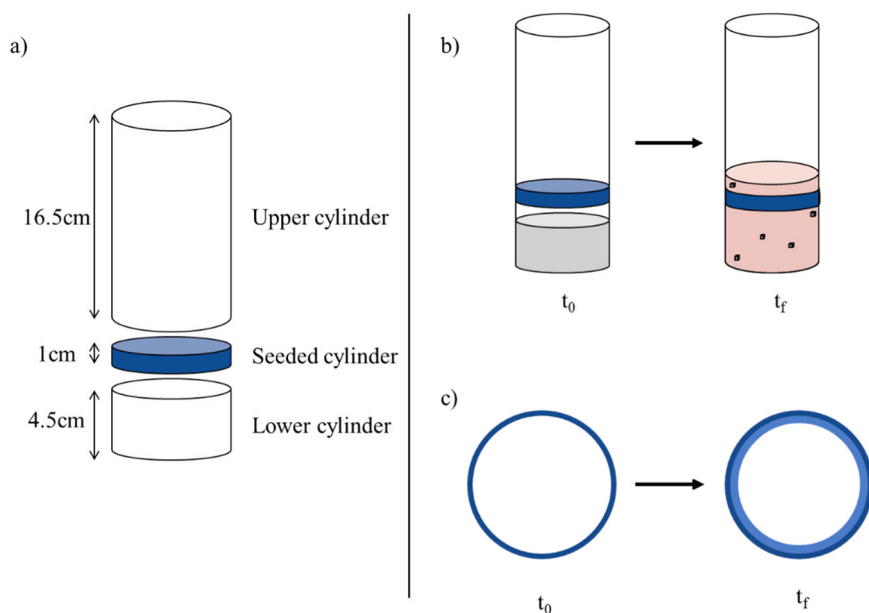
Fig. 3. Preferential crystallization principle. a) Set-up of the cylinder, with the seed material at a height of 4.5–5.5 cm, b) Evolution of the experiment over time, with the racemic initial solution in grey and the final solution, enriched in counter-enantiomer, in pink, c) Schematic theoretical crystal growth on the seeded cylinder at the end of the process, with the seed material in dark blue and the outcome of the crystallization in light blue.
