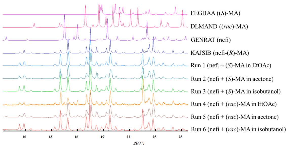
Fig. 2. Comparison of the XRPD patterns of nefi-(rac)-MA (1:1) cocrystallization through GAS in isobutanol (red), acetone (brown), EtOAc (orange), nefi-(S)-MA (1:1) cocrystallization through GAS in isobutanol (light green), acetone (dark green), and EtOAc (light blue), and the simulated patterns of the reported nefi-(R)-MA-cocrystal (CCDC refcode KAJISIB) [5] (dark blue) and parent compounds nefi (CCDC refcode GENRAT) [30] (violet), (rac)-MA (CCDC refcode DLMAND) [31] (magenta), and (S)-MA (CCDC refcode FEGHAA) [32] (pink).
