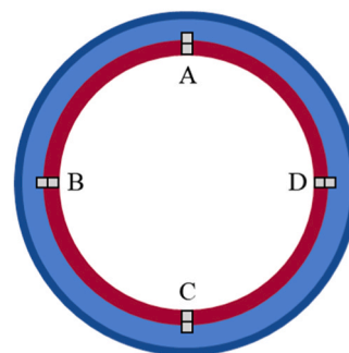
Fig. 4. Crystal growth occurs in layers on the seeded cylinder. As one moves away from the initial seed layer to the outer surface, the enrichment in nefi-(R)-MA becomes less pronounced. In dark blue, enantiopure seeding, e.g. nefi-(R)-MA; in light blue crystalline material still enriched in nefi-(R)-MA; in dark red, crystalline material enriched in counter-enantiomer, nefi-(S)-MA. The different samples taken are represented as grey squares.
