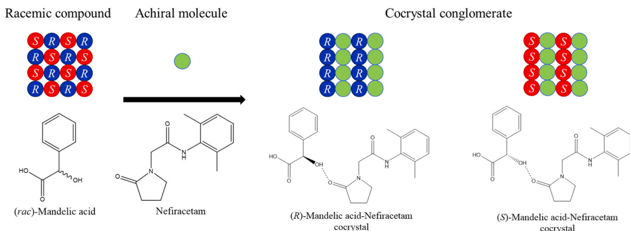
Fig. 1. Conversion of the racemic compound mandelic acid into a conglomerate through cocrystallization with nefiracetam.
