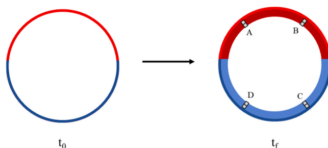
Fig. 5. Cylinder seeded on one side with nefi-(R)-MA (dark blue) and the other with the nefi-(S)-MA (light red). Over time, a layer half enriched in nefi-(R)-MA (light blue) and half in nefi-(S)-MA (dark red), grows. The different samples taken are represented as grey squares.
