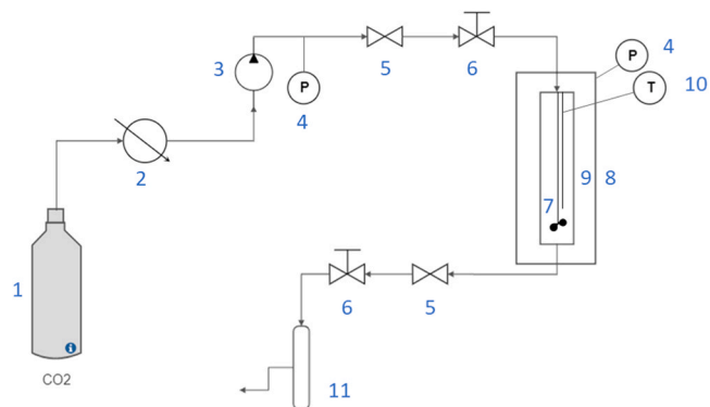
Scheme 1. GAS set-up, with 1. \text{CO}_2 tank; 2. cooler; 3. \text{CO}_2 pump; 4. pressure gauge; 5. valve; 6. metering valve; 7. mechanical stirrer; 8. reactor; 9. glass cylinder; 10. thermocouple; 11. outlet collector.
