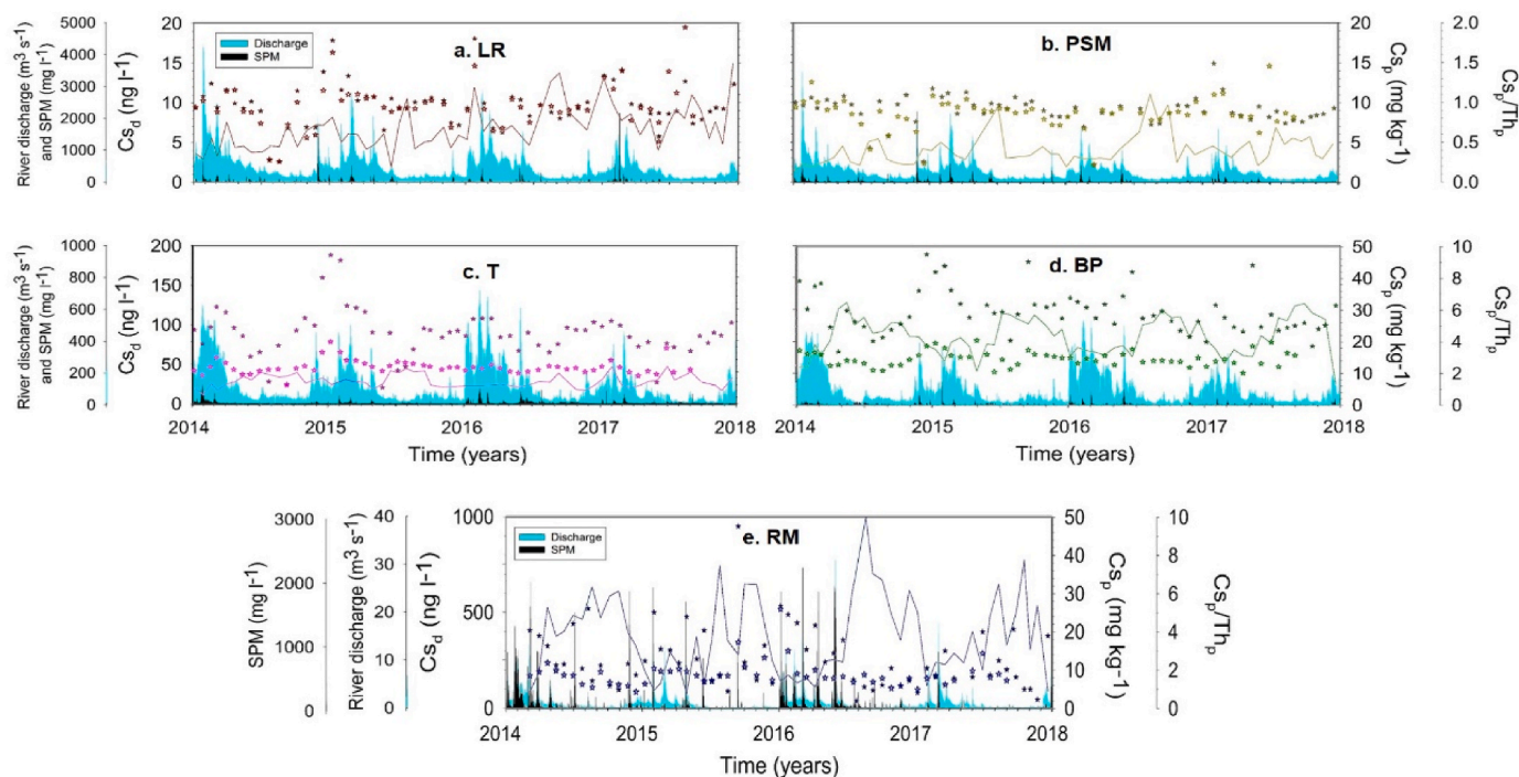
Fig. 3. Temporal variability of dissolved ( C_{sd} – lines), particulate ( C_{sp} – filled stars) and Th-normalized ( C_{sp}/Th_p – empty stars) cesium (Cs) concentrations in the Lot-Garonne fluvial system from 2014 to 2017 (4-years) at five sampling sites: La Réole (a, LR_Gar-70km), Port-Sainte-Marie (b, PSM_Gar-135km), Temple (c, T_Lot-135km), Boisse-Penchat (d, BP_Lot-235km) and Riou Mort (e, RM_Rio-250km). Corresponding water discharges are blue-shaded areas and suspended particulate matter (SPM) concentrations are also included. (For interpretation of the references to colour in this figure legend, the reader is referred to the Web version of this article.)
