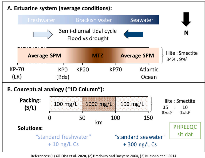
Fig. 2. Schematic parallelism between (A) the physical-chemical characteristics of the Gironde Estuary and equivalent kilometric points (KP), and (B) the conceptual 1D column used to numerically simulate the adsorption of Cs along a salinity and turbidity gradients. Abbreviations: solid to liquid ratio (S/L), cation exchange (Exch.).
