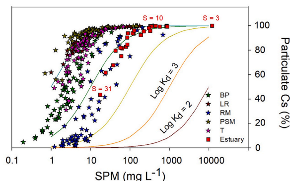
Fig. 10. Distribution of the C_{sp} content (%) out of the total Cs in the samples along the SPM concentrations in the Lot-Garonne-Gironde fluvial-estuarine system during 4-years of monitoring (stars) and 2 hydrological conditions (squares) along the salinity gradient (i.e., indicated in red). The corresponding salinities for the estuarine points are also included. Fluvial sites correspond to: La Réole (LR_Gar-70km), Port-Sainte-Marie (PSM_Gar-135km), Temple (T_Lot-135km), Boisse-Penchot (BP_Lot-235km) and Riou Mort (RM_Rio-250km). Estuarine values were calculated from the results between Bdx 0 km and C_110 km. (For interpretation of the references to colour in this figure legend, the reader is referred to the Web version of this article.)
