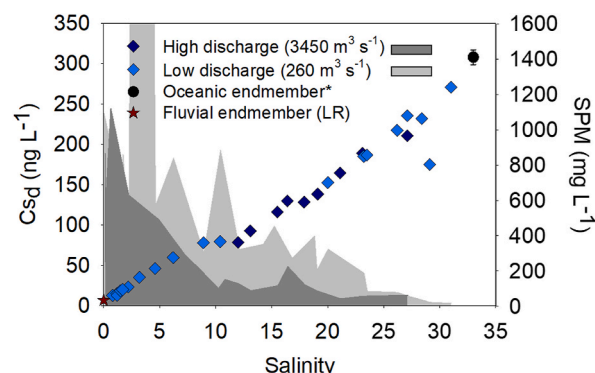
Fig. 4. Distribution of C_{sd} (symbols) along the salinity and turbidity (shaded areas) gradients of the Gironde Estuary in flood (MGTS II – March 2015, 3450 \text{ m}^3 \text{ s}^{-1} ) and drought (MGTS III – October 2015, 260 \text{ m}^3 \text{ s}^{-1} ) conditions, sampled between the city of Bordeaux (Bdx_0 km) and the estuary mouth (C_110 km). Freshwater endmember is calculated from the 4-y timeseries at LR_Gar-70km (i.e., Fig. 3, error bar smaller than the symbol size) and the oceanic endmember corresponds to reported values in the literature (Rankin, 2009; Takata et al., 2013). Gray areas represent the SPM concentrations of corresponding campaigns.
