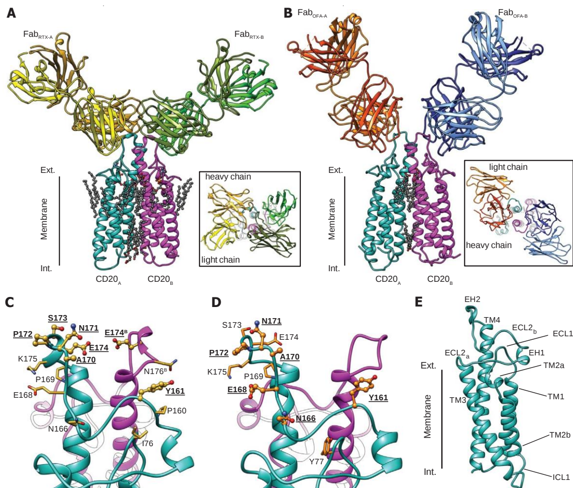
Fig. 3. Structures of CD20 complexes with type I Fab fragments. (A and B) Structures of CD20 in complexes with two Fab RTX -bound (A) and Fab OFA -bound (B) molecules, color coded as in Fig. 2, D to F. Insets show extracellular views of the Fab variable domains bound to CD20. (C and D) The most important CD20 residues interacting with single Fab RTX-A (yellow; C) or Fab OFA-A (orange; D) molecules are highlighted. Residues in ball-and-stick representation establish the majority of H-bonds and contacts with the Fab molecule. Single-letter abbreviations for the amino acid residues are as follows: A, Ala; C, Cys; D, Asp; E, Glu; F, Phe; G, Gly; H, His; I, Ile; K, Lys; L, Leu; M, Met; N, Asn; P, Pro; Q, Gln; R, Arg; S, Ser; T, Thr; V, Val; W, Trp; and Y, Tyr. (E) Membrane view of CD20 A subunit from the CD20-Fab RTX complex.
