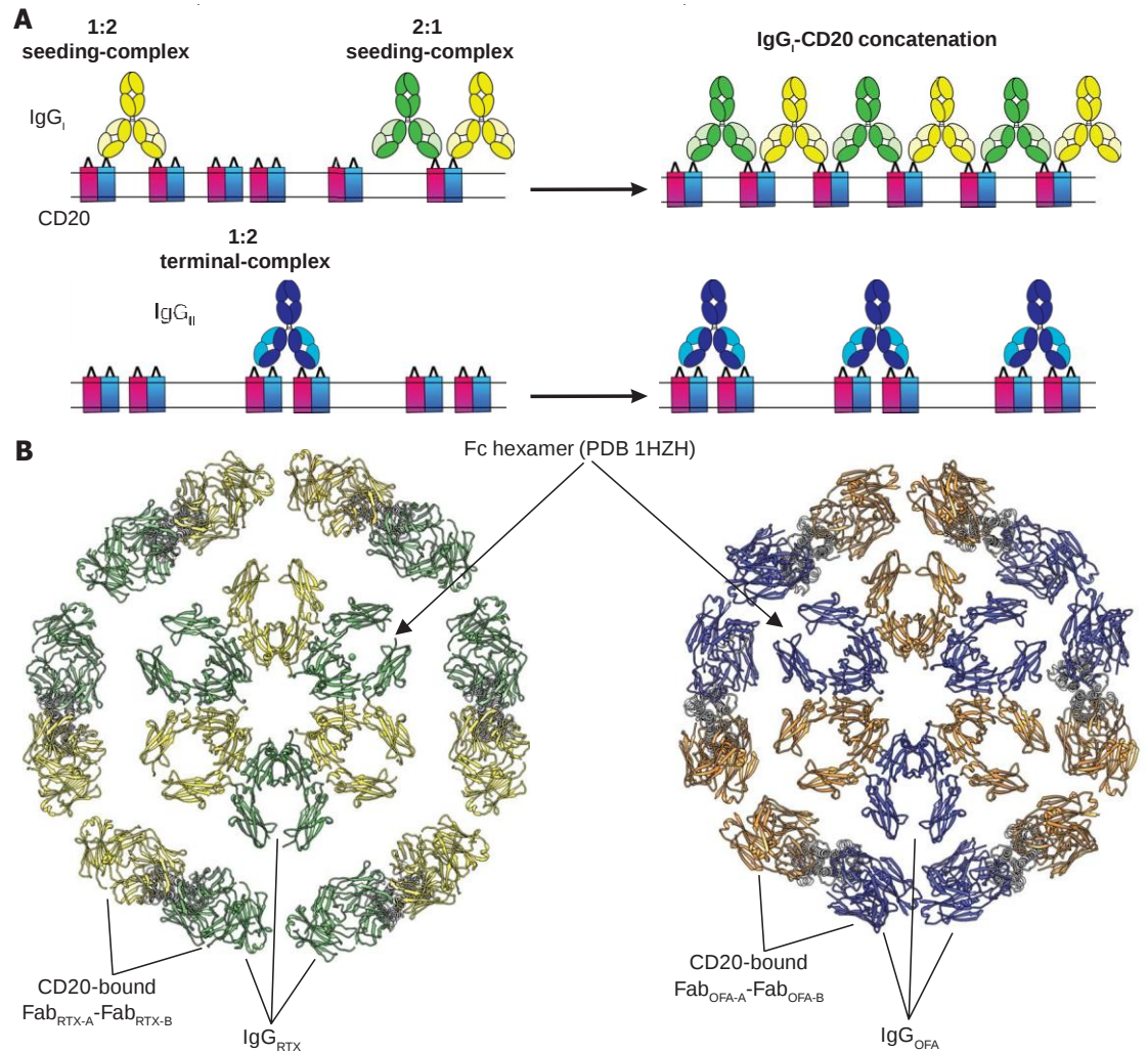
Fig. 5. Binding mechanism and hexameric CD20-IgG model. (A) IgG:CD20 seeding and terminal complex mechanisms for type I and II mAbs, respectively. (B) Extracellular view of a structural model built with the symmetric Fc hexamer from PDB 1HZH and six copies of CD20-Fab RTX (left) or CD20-Fab OFA (right) structures (determined in this work), arranged symmetrically and concentric to the Fc ring. The space between CD20-Fab complexes was minimized to avoid clashes between Fab domains bound to different CD20 molecules. Fc domains and the two corresponding Fab domains are shown in the same color.
