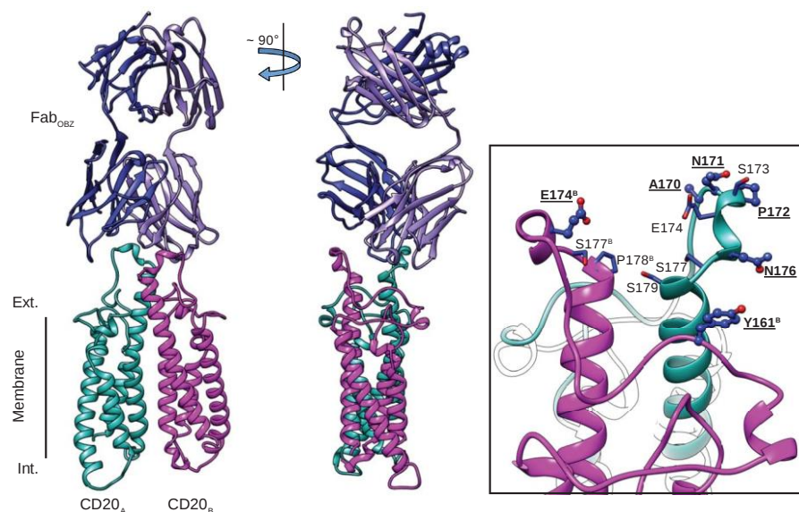
Fig. 4. Structure of CD20 in complex with type II Fab OBS . Structure of CD20 with one Fab OBS -bound molecule. Fab OBS interacts more extensively with CD20 A subunit (cyan), but it also interacts with CD20 B (pink). Inset shows the most important CD20 residues interacting with Fab OBS . Residues in ball-and-stick representation establish the majority of H-bonds and contacts with the Fab molecule.
