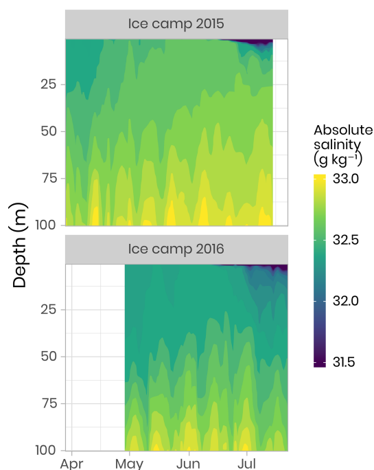
Figure 3. Temporal evolution of the salinity in the first 100 m of the water column for both campaigns. Note that, for visualization purposes, salinity below 31.5 \text{ g kg}^{-1} has been binned to 31.5 \text{ g kg}^{-1} . Note that salinity as low as 4 \text{ g kg}^{-1} was observed during flushes of freshwater at the ocean surface due to snow and ice melt (dark blue color in the figure).
