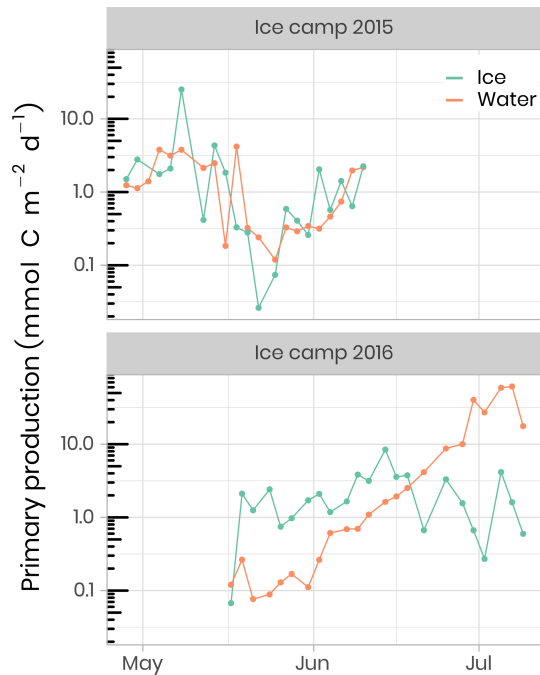
Figure 11. Temporal evolution of primary production in ice and water (depth-integrated) for both ice camp missions.
