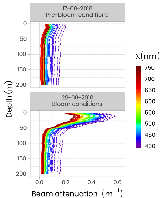
Figure 7. Beam attenuation coefficients ( c , \text{m}^{-1} ) measured in 2016 using a WetLabs AC-S before and during the phytoplankton bloom. Note that the colors of the lines correspond to wavelength frequencies.
