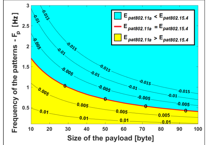
Figure 6. The Equal-energy curve of the 802.11a and 802.15.4 in the proposed scenarios.
