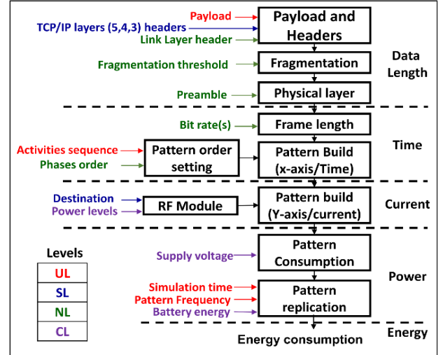
Figure 3. An energy-aware cross-level model for RF activities.
