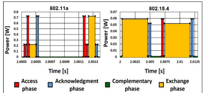
Figure 4. Energy consumption patterns for different wireless link protocols (Node B, Payload length = 100 Bytes, F_p = 1 Hz).
